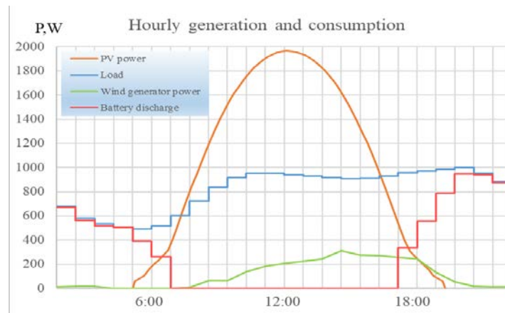
Figure 10. Battery storage expected working cycle.
