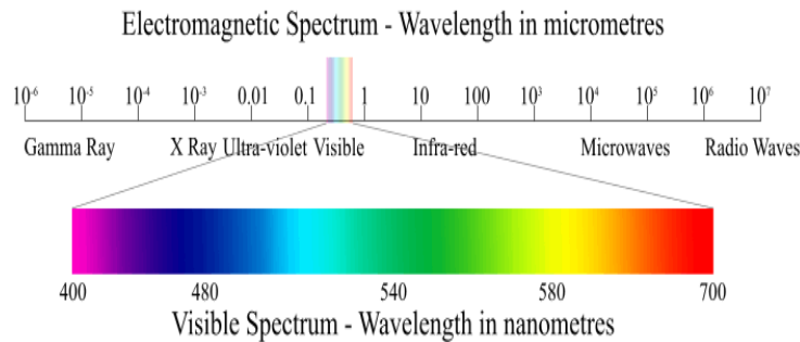
Figure 1. Visible range of electromagnetic spectrum.
