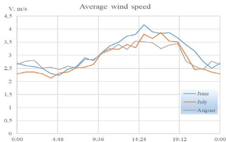
Figure 9. Hourly wind profiles for each summer month.
