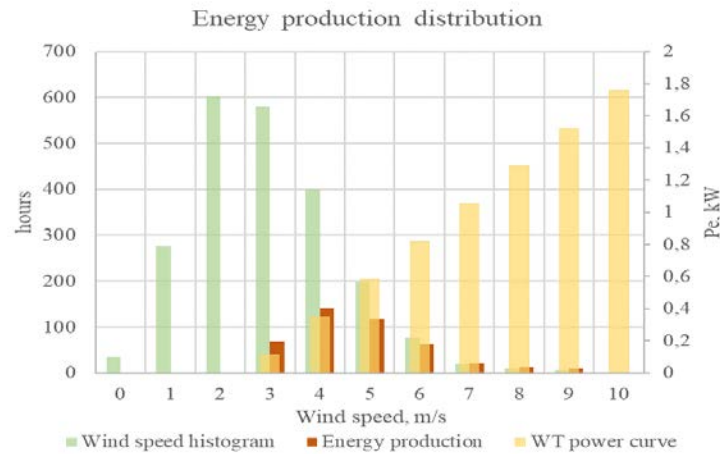
Figure 8. Wind turbine power curve wind speed and energy production distribution.
