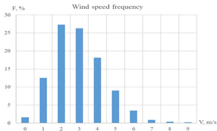
Figure 7. Dominant wind speed values at the selected site.
