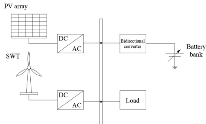
Figure 4. Simplified representation of an autonomous grid
