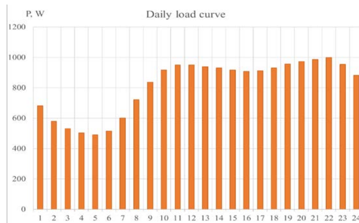
Figure 5. Total daily load curve.
